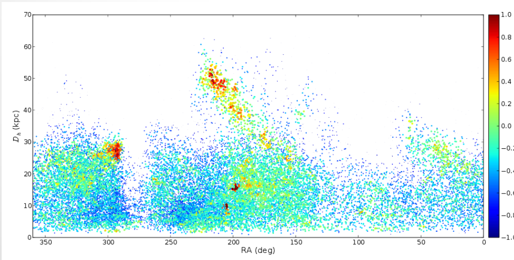
RR Lyrae as line of sight resolvers
