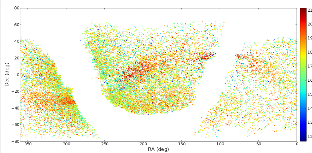
Catalina RR Lyrae coverage
