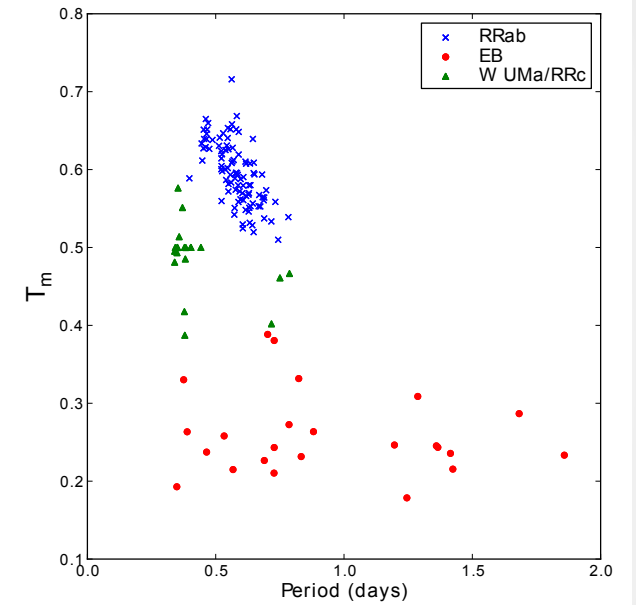
Simple statistic to discriminate
